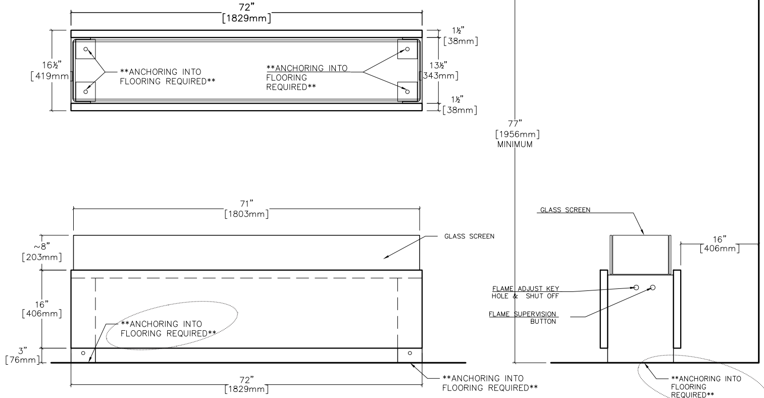
CLEARANCES to ADJACENT MATERIALS
