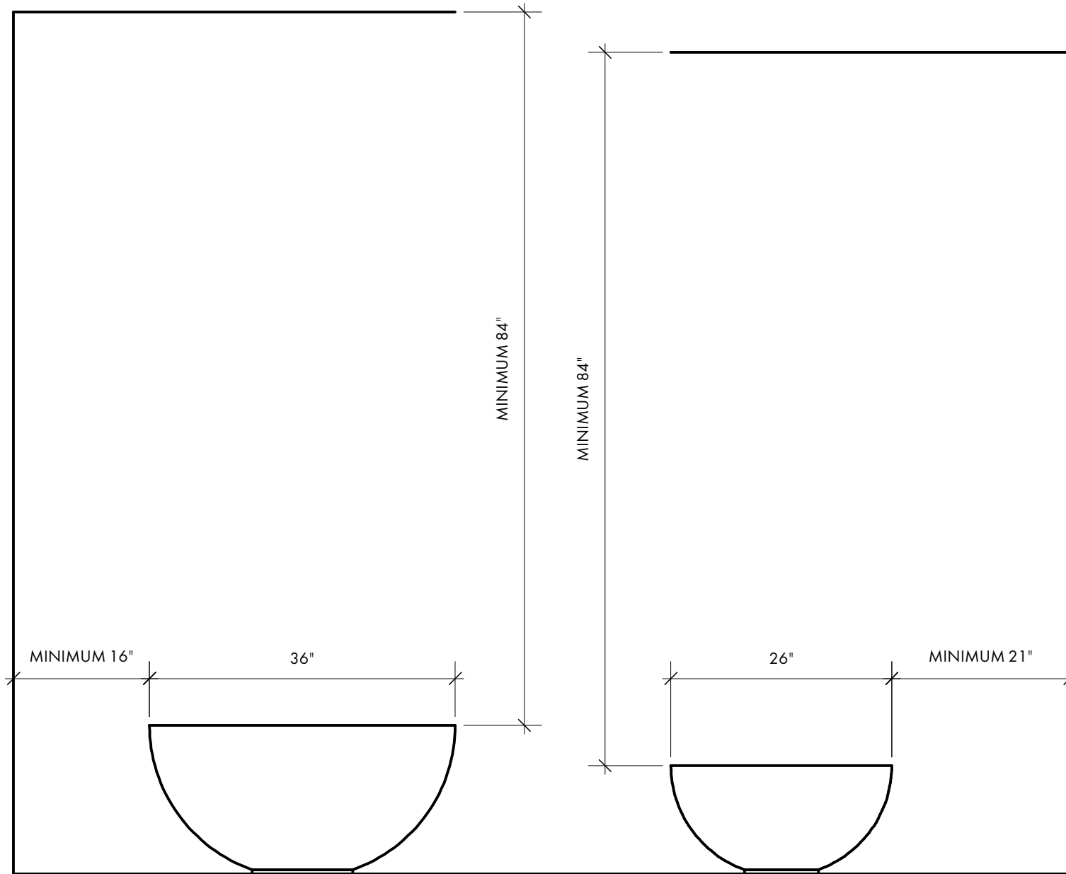
FIREBOWL - Mininim Distances to Combustibles Scale: 3/4" = 1'-0"
